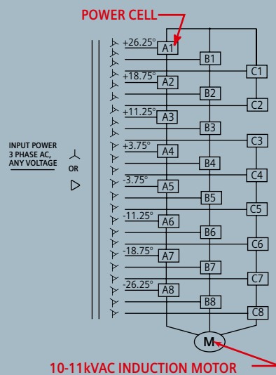
10-11kVAC INDUCTION MOTOR 10-11kV 变频器拓扑
